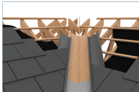
Slate Roof Valley Trim >> CONTEXT VIEW
